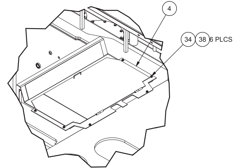
DETAIL 1C
