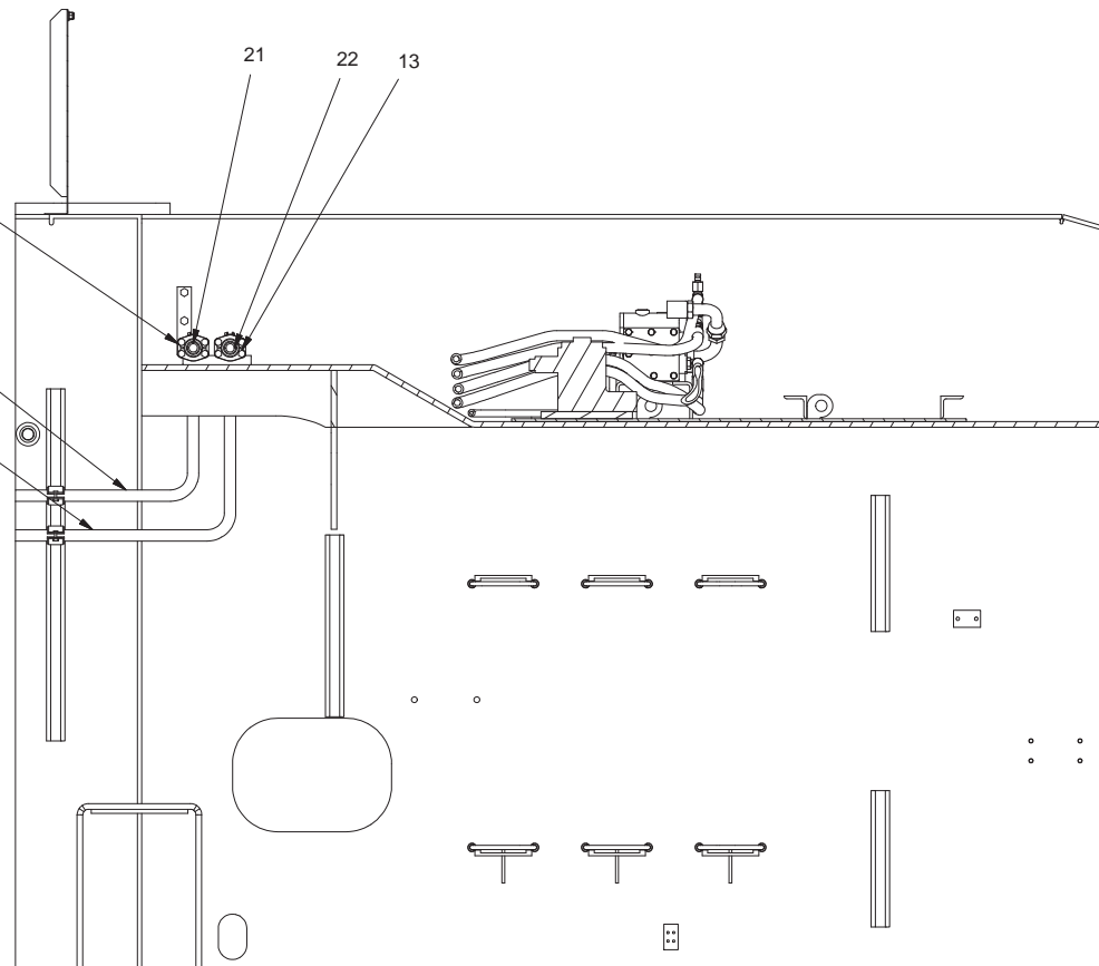
SECTION B-B
