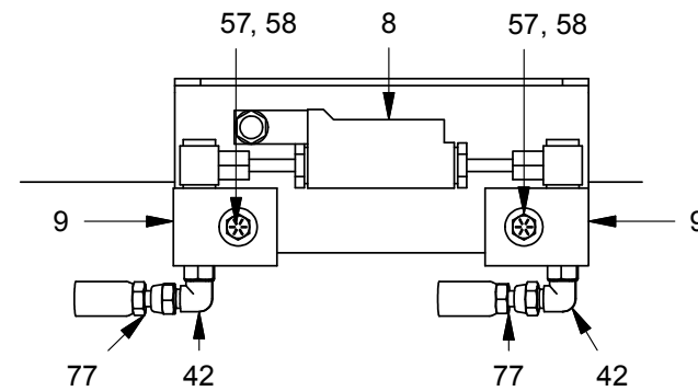
SECTION G-G
