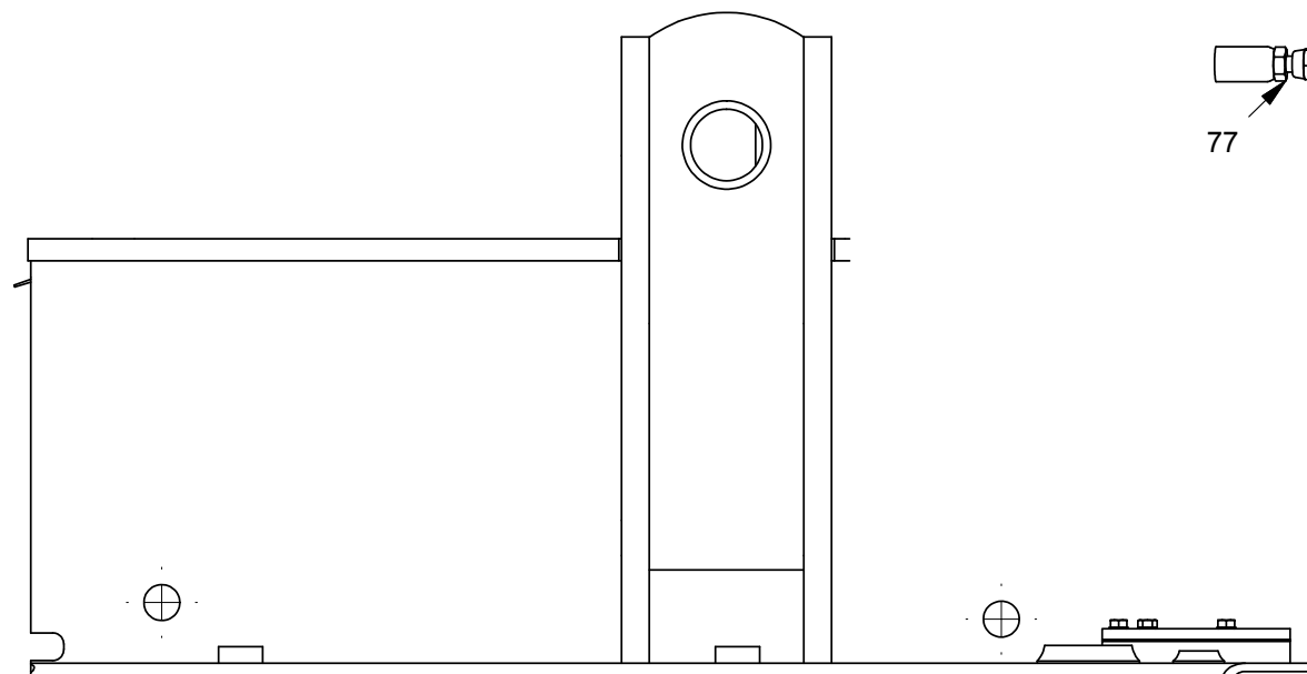
SECTION G-G
