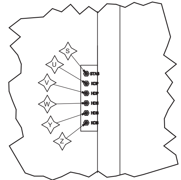
DETAIL B W/ NO OR LWR AUX HLDWN
