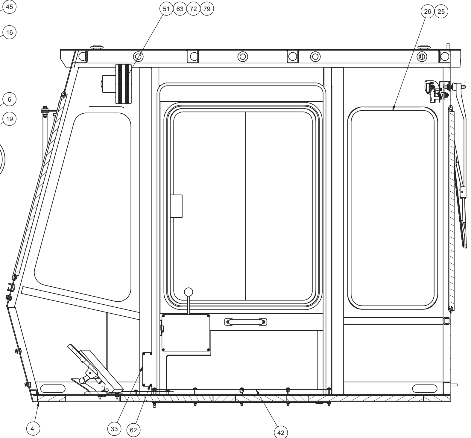
SECTION E-E
