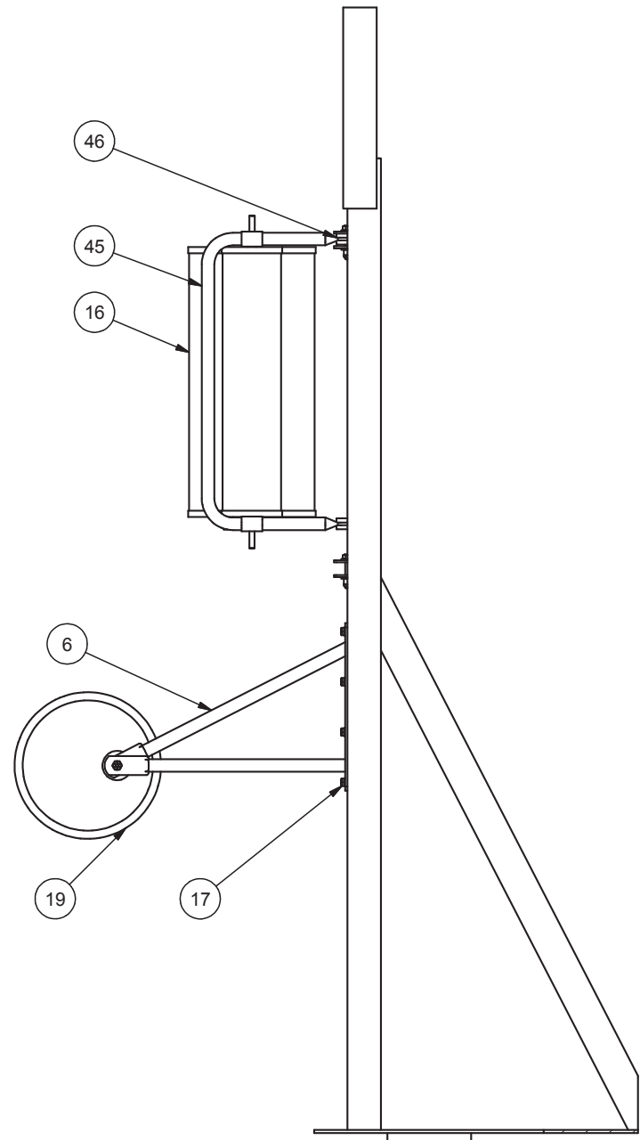
SECTION K-K
