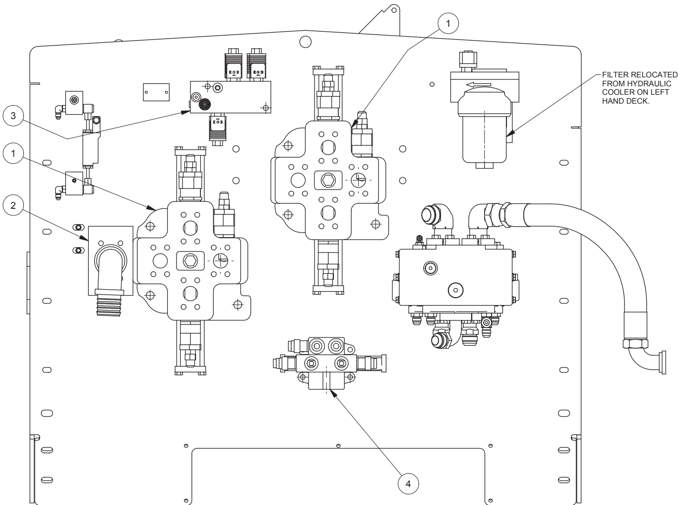
VALVE LAYOUT
