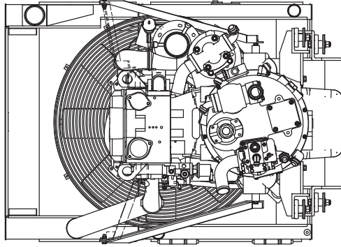
VIEW B-B SCALE 0.08 : 1
