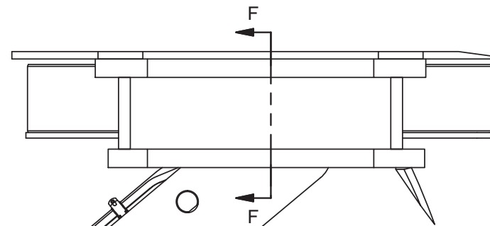
DETAIL E
