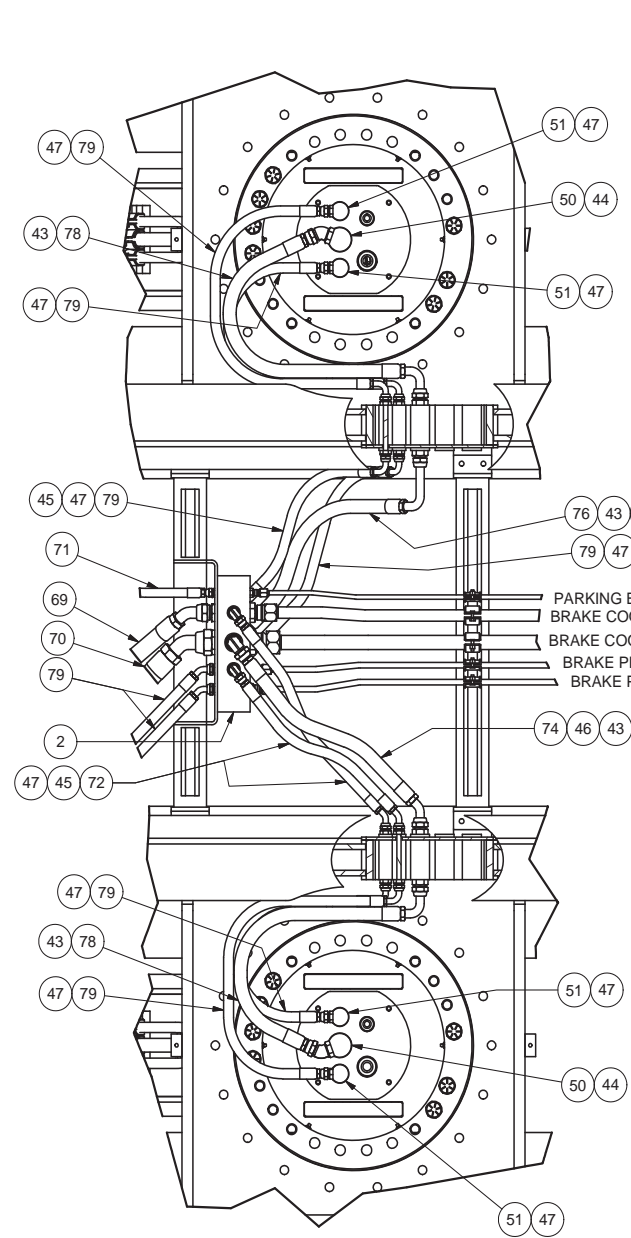
DETAIL A
