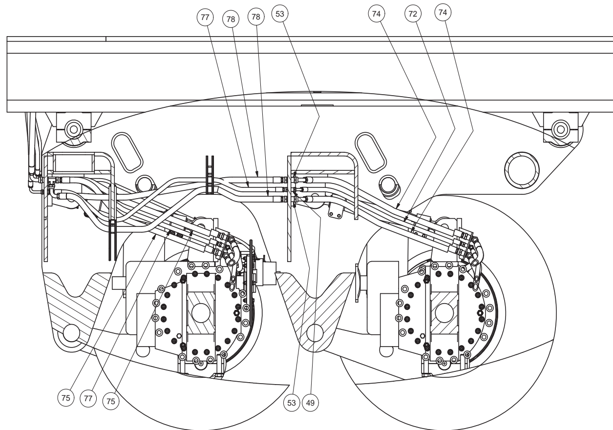
VIEW G-G
