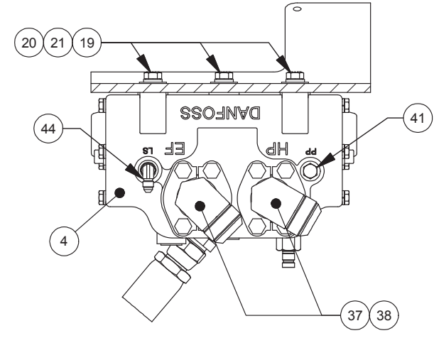
VIEW ON E-E
