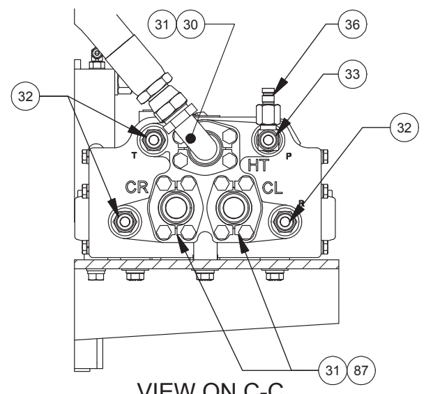
VIEW ON C-C
