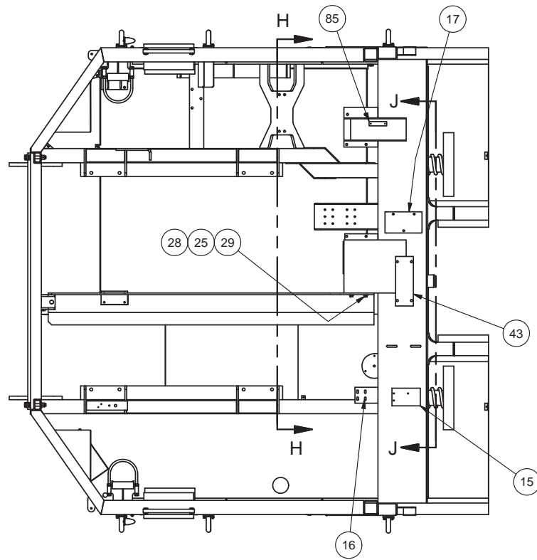
VIEW L-L
