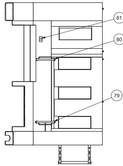
SECTION K-K
