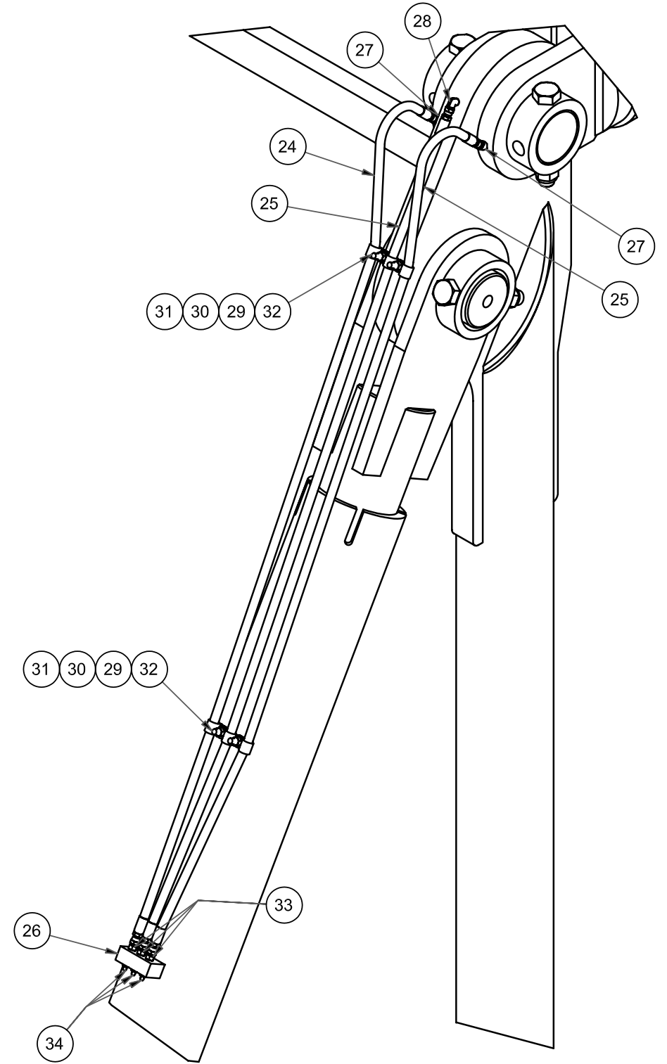
DETAIL E
