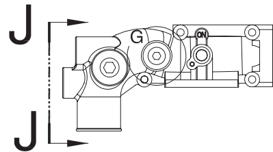
DETAIL G
