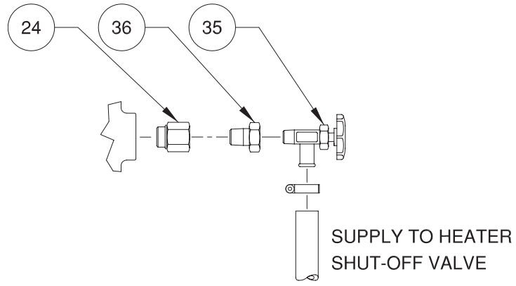
2 DETAIL G VIEW J-J HEATER SUPPLY (DETAIL F: HEATER RETURN, SIMILAR)
