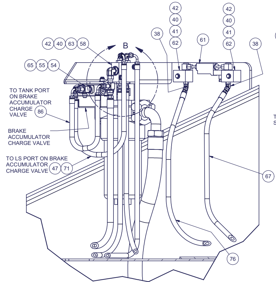
DETAIL A
