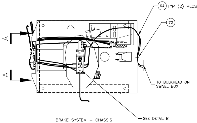
BRAKE SYSTEM - CHASSIS
