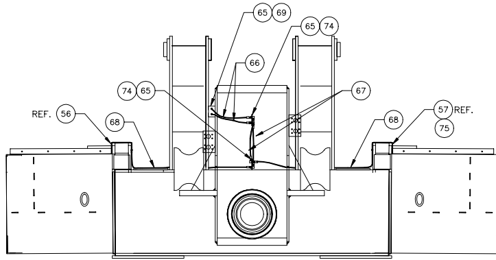
BRAKE SYSTEM - BOGIE
