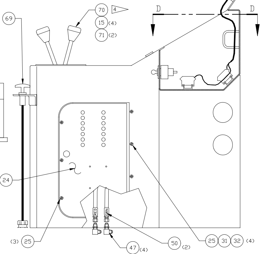
CONSOLE VIEW A-A
