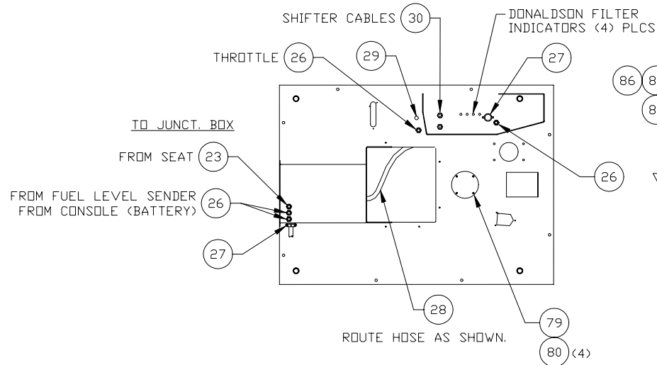
FLOOR PLATE VIEW B-B CUTOUT DESIGNATIONS
