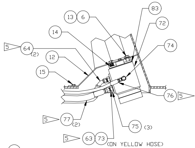
VIEW C-C
