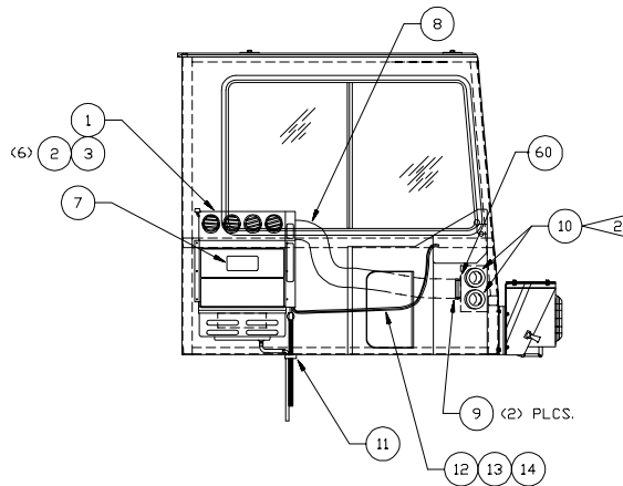
VIEW B-B CAB INTERIOR, LEFT SIDE
