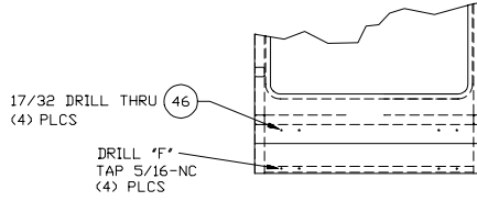
VIEW F-F COWL EXTERIOR, LEFT SIDE
