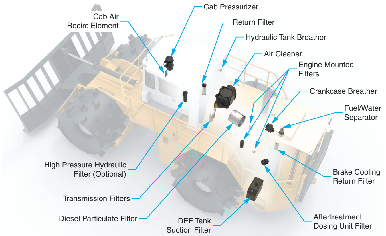
Figure 1 Filter Arrangement
