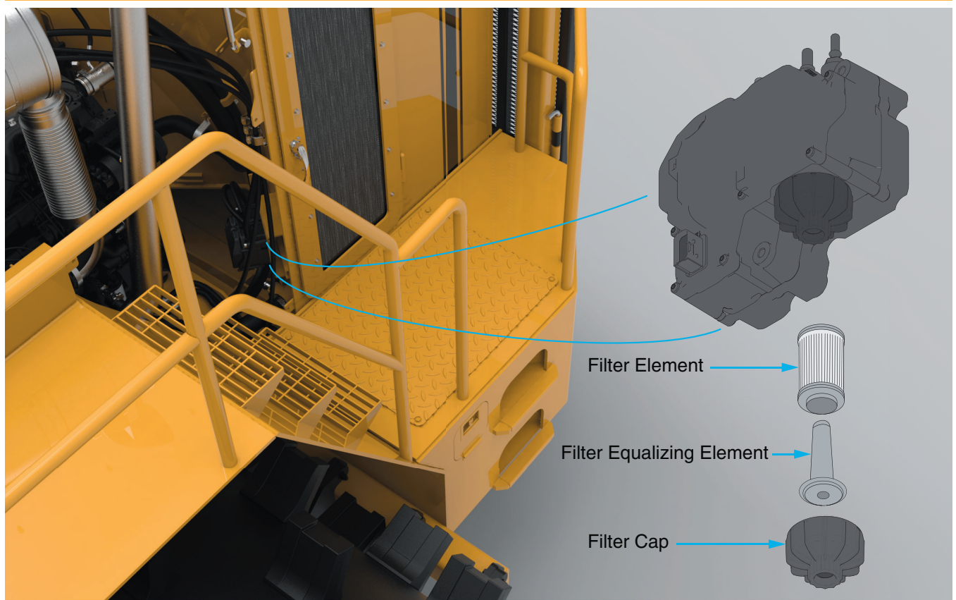
Figure 28 Aftertreatment Dosing Unit Filter
