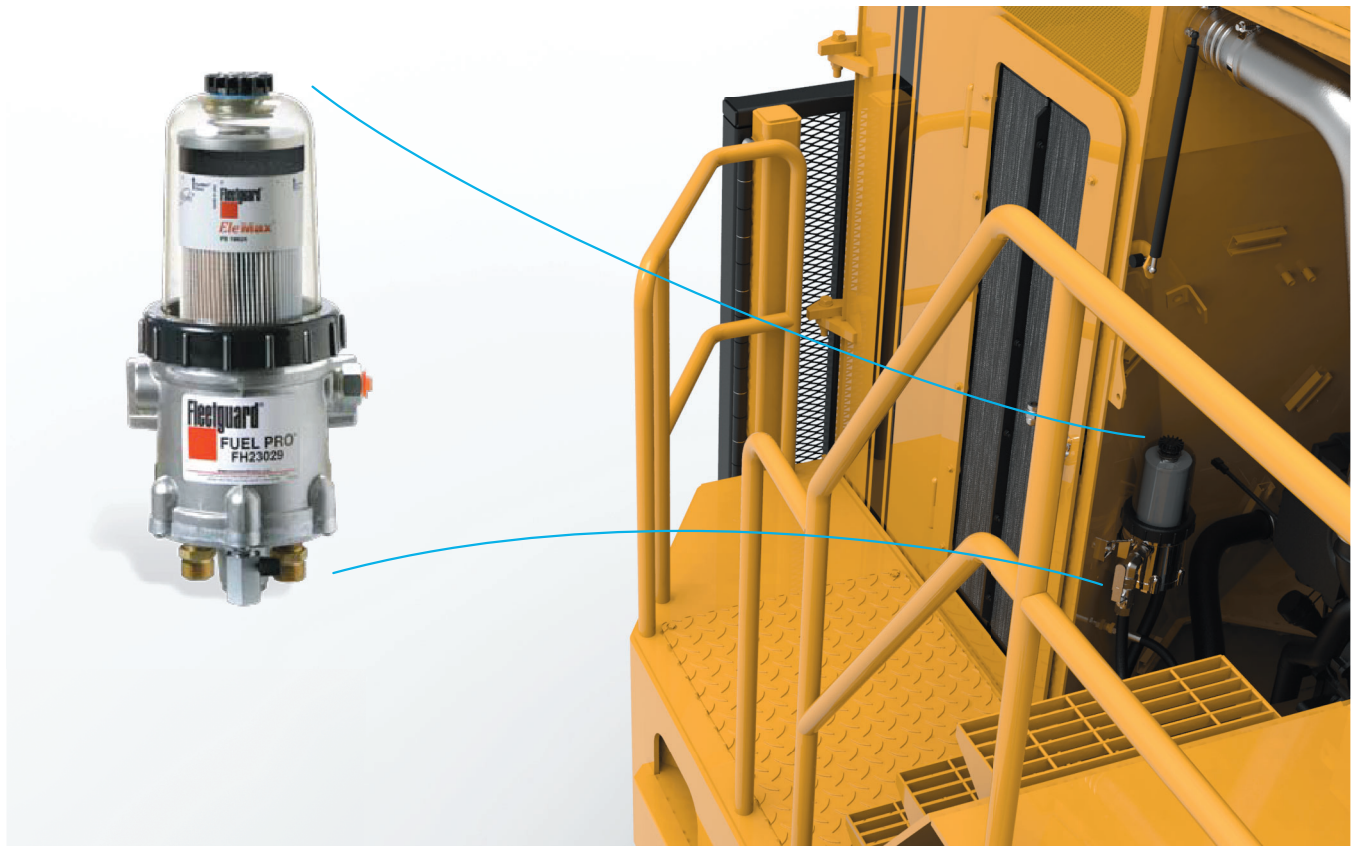
Figure 19 Fuel/Water Separator
