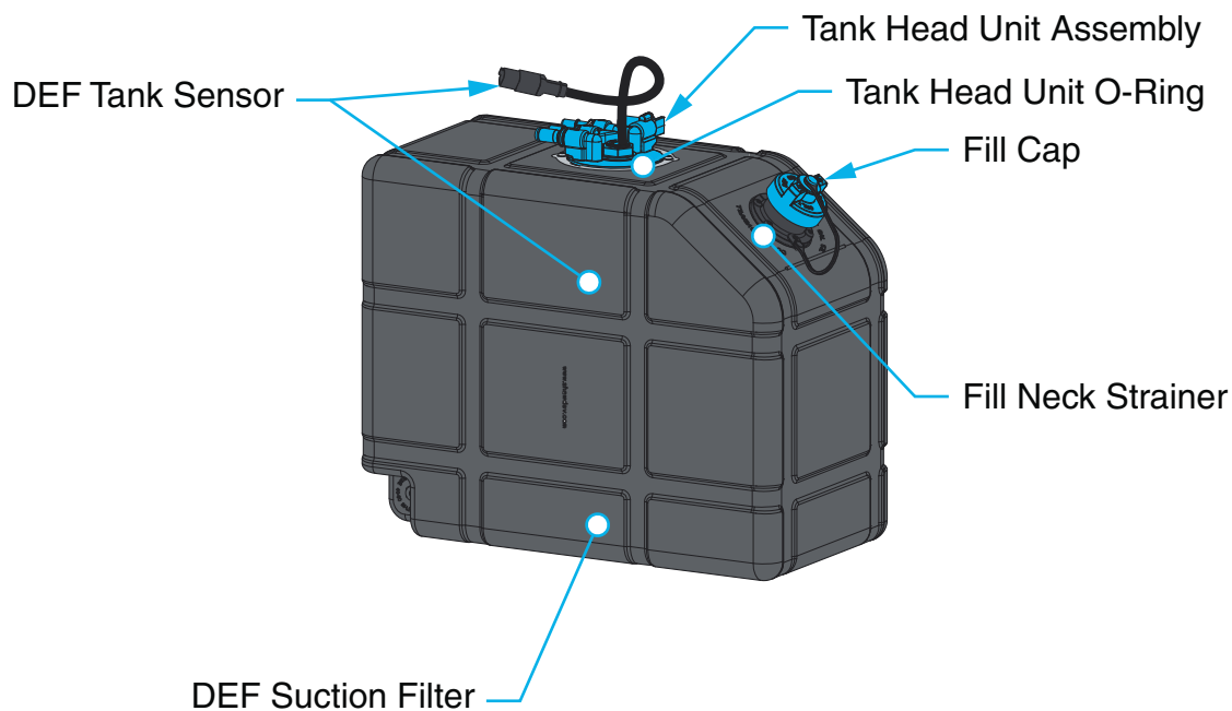
Figure 27 DEF Tank
