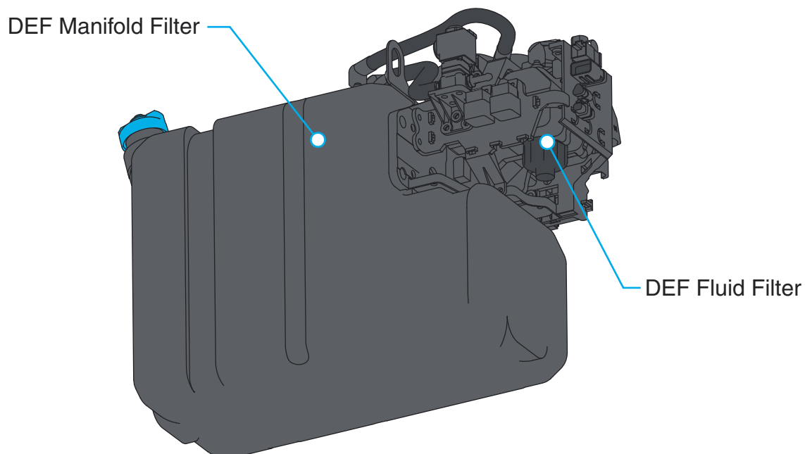
Figure 13 DEF Tank
