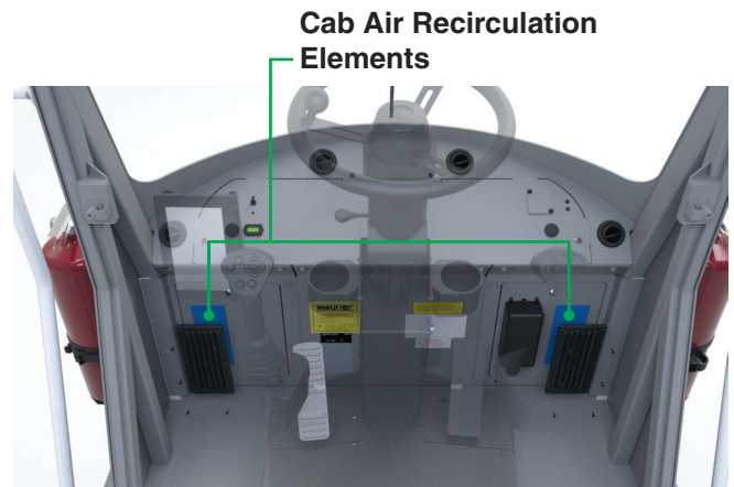
Figure 16 Cab Air Recirculation Elements
