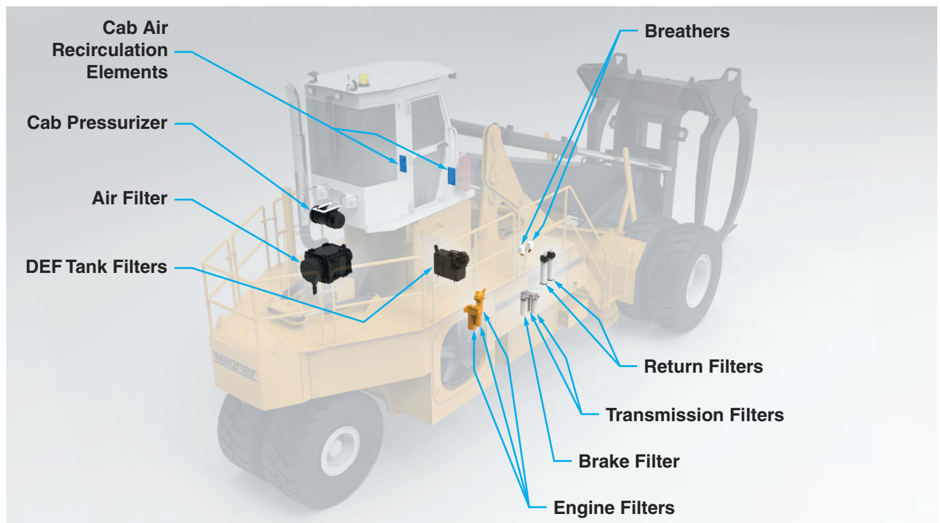
Figure 1 Filter Arrangement
