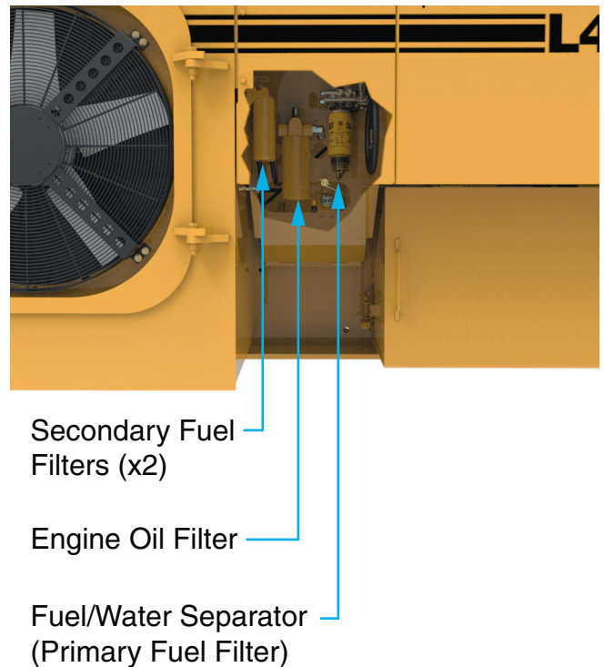
Figure 6 Engine Filters
