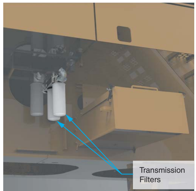
Figure 7 Transmission Filters
