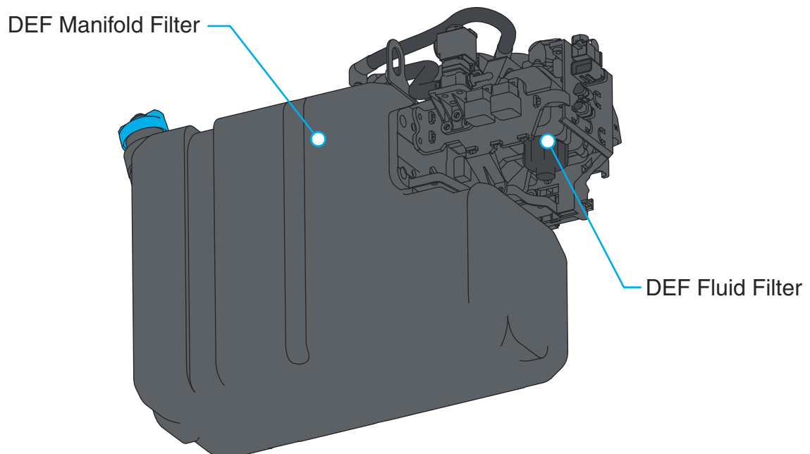
Figure 10 DEF Tank
