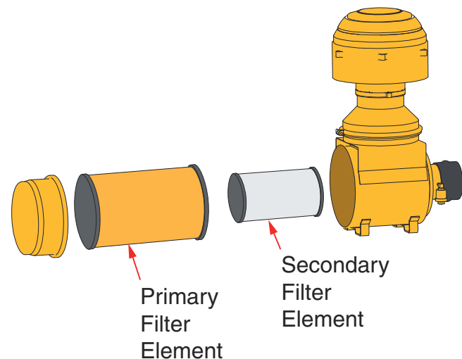
Figure 9 Air Cleaner Elements
