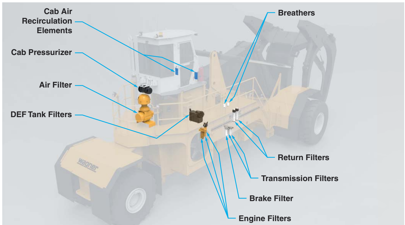
Figure 1 Filter Arrangement
