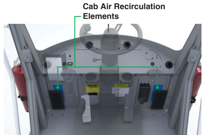
Figure 13 Cab Air Recirculation Elements
