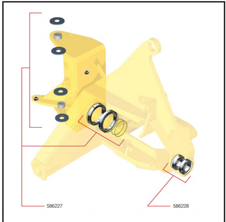
Figure 1. Service Kits
