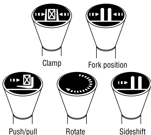
Figure 2-5, Operator controls
