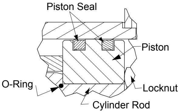
Figure 3-5, Piston Seal
