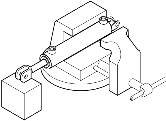
Figure 3-1, Cylinder Vise
