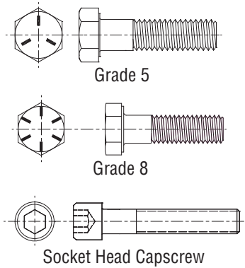
Figure 4-1, Bolt Identification
