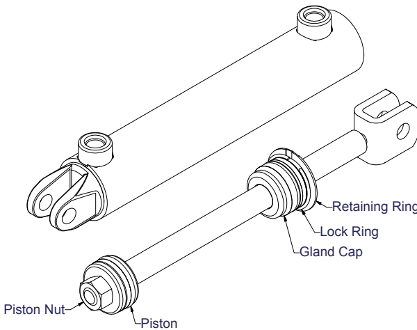
Figure 3-2, Cylinder Rebuild
